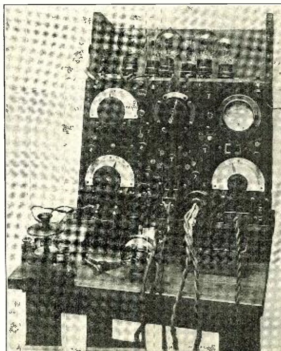
Fig. 4. In This Case We Have a Complete Transmitter-Receiver Field Set Suitable for Small Wavelengths from 250 to 650 Meters.
