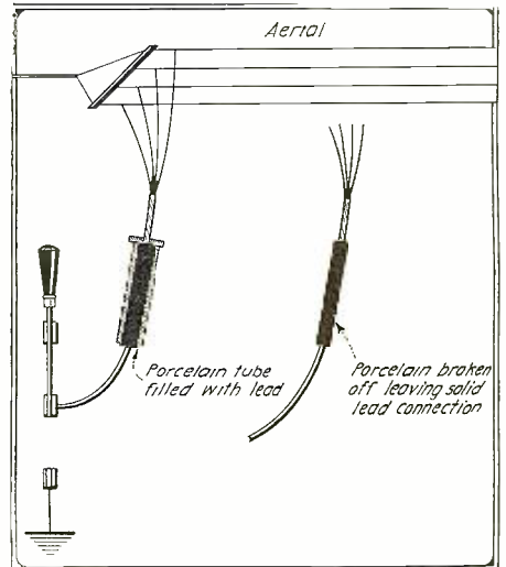
If This Idea is Followed Out You Will Experience no Future Trouble With Loose or Grinding Lead-in Contacts.
