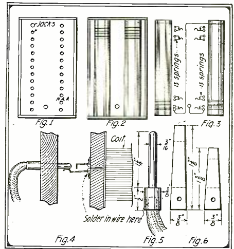
If You Are Looking for an Efficient Loading Coil, Doing Away With "Dead" Ends, Follow Out These Directions.
