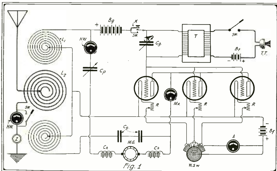
This Diagram Shows the Schematic Hook-up of the Set and Is One taken from Leading Text Books and Magazines. It is a Circuit of High Power and a Persistent Oscillator.
