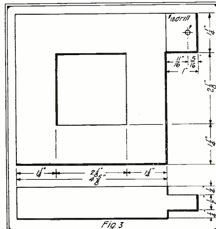
In This Sketch We Have the Dimensions of the Core Laminations With Projecting Lug. These Should Preferably Be of Silicon Steel.
