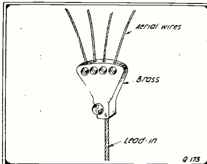
This Four Wire Aerial Lead-In Connector May Be Easily Made at Short Notice
