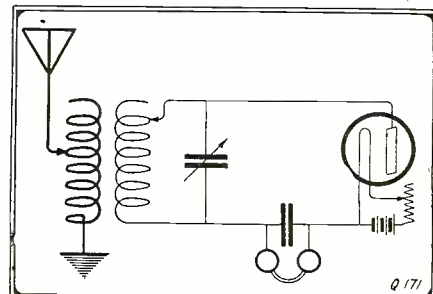
A Simple Two Element or Fleming Valve Detector Circuit.
