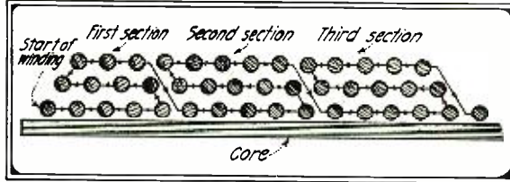
This Diagram Shows An Imaginary Cross Section of One Side of a Coil Having Three Layers and at the Same Time Gives You an Idea Just How to Go About the Winding Process.
