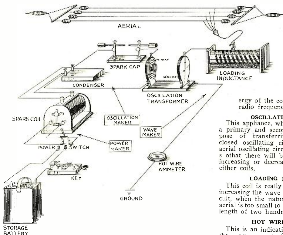
Fig. 3. This Illustration Shows a Perspective of the Transmitting Instruments Actually Hooked Up Ready for Work. The Ground of Course, Should Be Connected to a Water Pipe or Any Other Form of Ground Connection.
