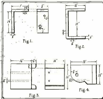
These Four Figures Represent Construction Details of the Various Necessary Parts.
