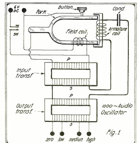
Complete Circuit Diagram of the Audio Oscillator.
