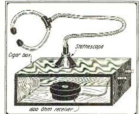
If Your Father is a Doctor Don't Appropriate His Best Stethoscope—Ask for an Old One.
