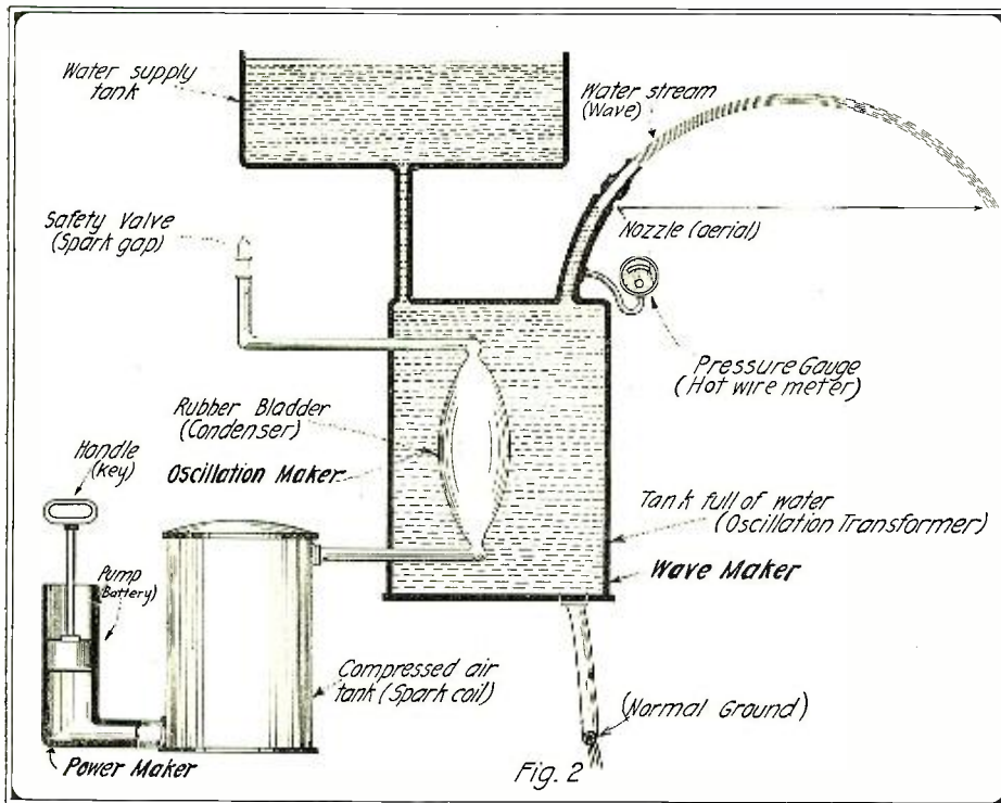
This Analogy Shows What May Be Assumed to Take Place in a Regular Spark Coil Transmitter. Study It Closely in Connection with This Article
