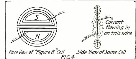
Two Coils in Series With the Fields Opposing Form a "Figure 8" Coil, as Shown Here.
