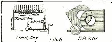
This Shows the Construction of a Transmitting Type of Variometer. Note the Coupling Arrangement.
