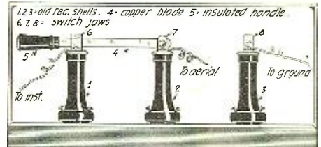
Be Sure to Fasten the Old Receiver Shells to the Base in a Secure Manner.
