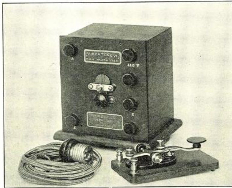
Here is Just the Transmitter for the Beginner to Start With. No Inductances, No Condensers, No Spark Gap to Bother With. Connect It to the House Lighting System and "Shoot" Away.
