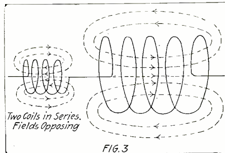
Direction of Lines of Force of Two Coils in Series With Fields Opposing.
